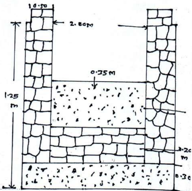
CROSS SECTION
